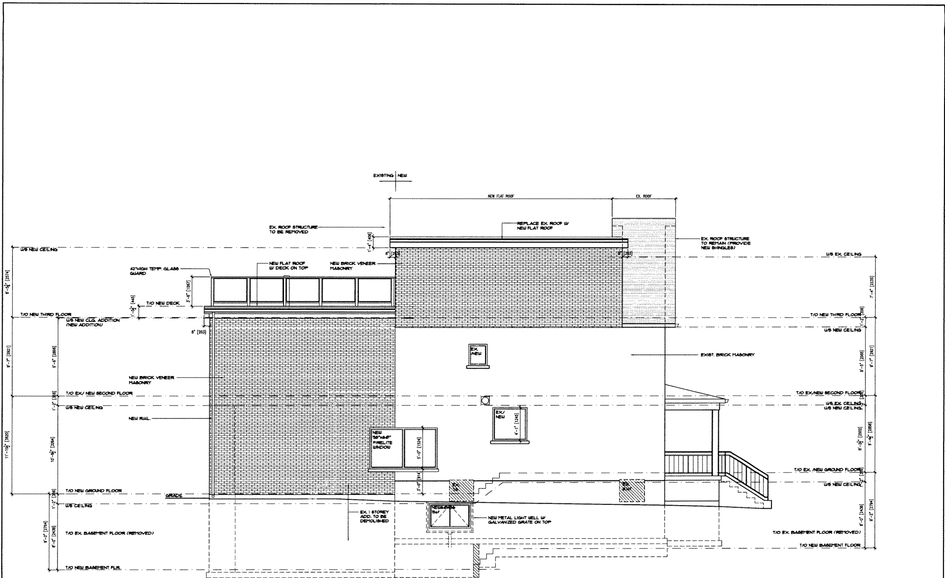
1 NORTH ELEVATION A6
